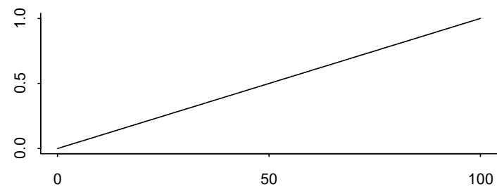
Point transect
